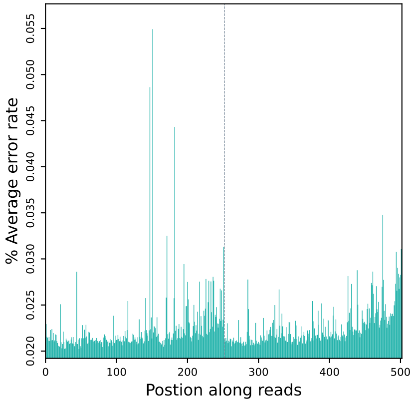
Error rate distribution along reads (R10913)
